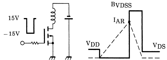
TEST CIRCUIT
