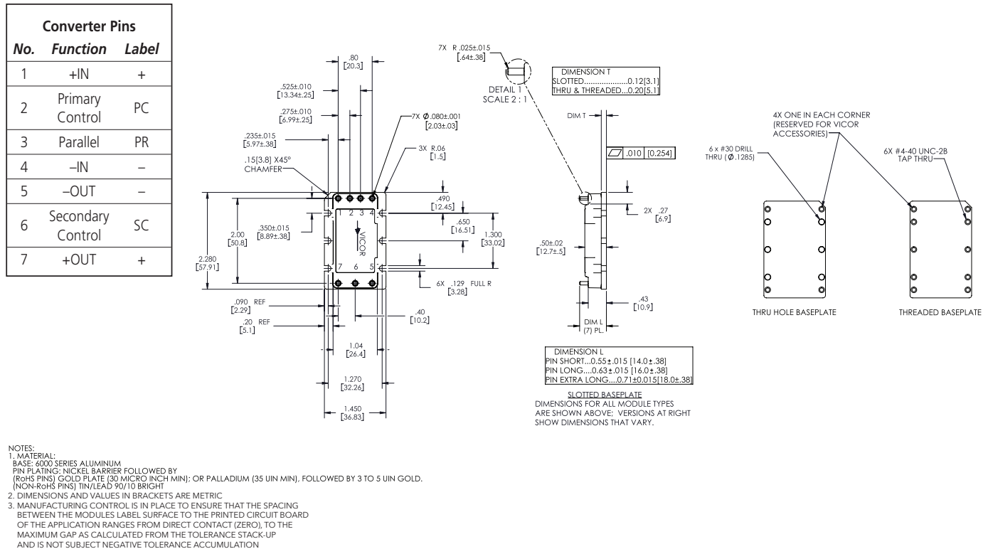
Figure 13 — Module outline
