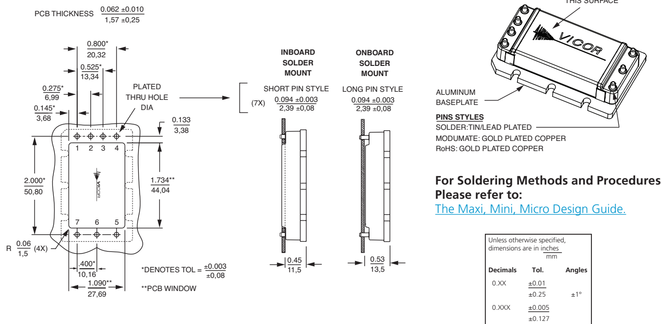
Figure 14 — PCB mounting specifications
