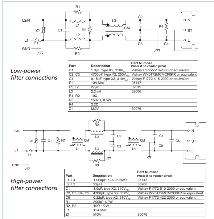
Figure 13 — Filter connections
