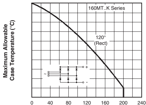
Fig. 6 - Current Ratings Characteristic
