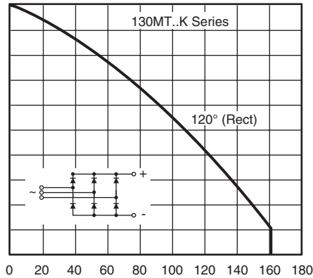
Fig. 1 - Current Ratings Characteristic
