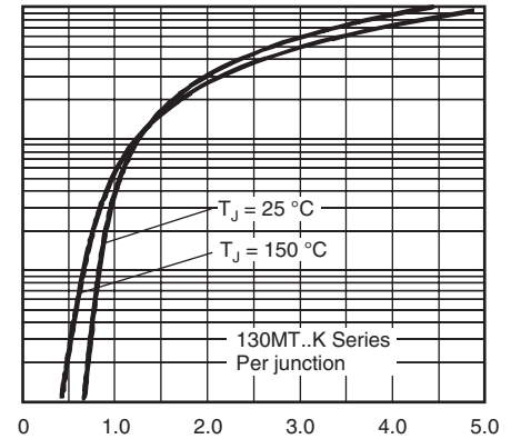
Fig. 2 - Forward Voltage Drop Characteristics
