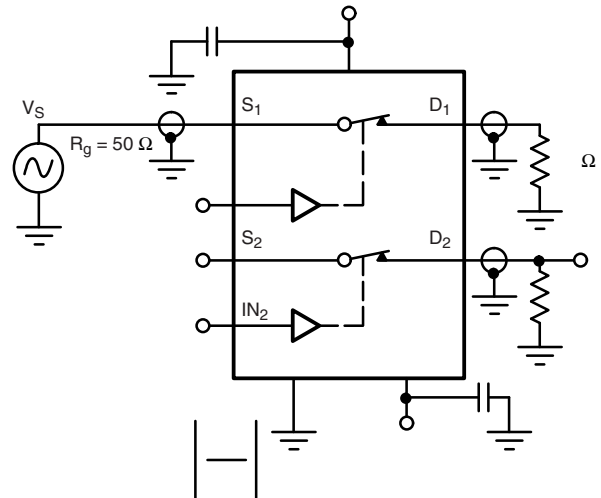
Figure 4. Channel-to-Channel Crosstalk
