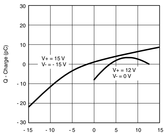
Q_S , Q_D - Charge Injection vs. Analog Voltage
