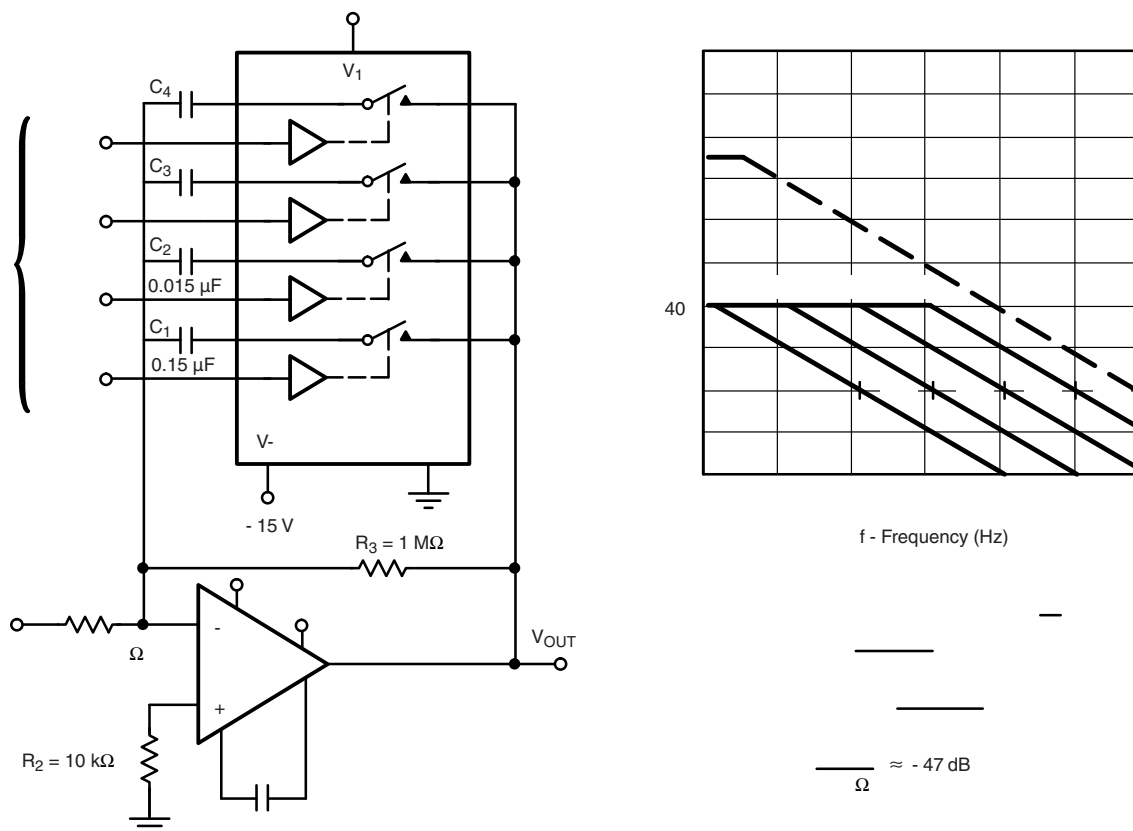
Figure 7. Active Low Pass Filter with Digitally Selected Break Frequency
