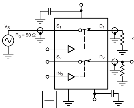
Fig. 4 - Channel to Channel Crosstalk
