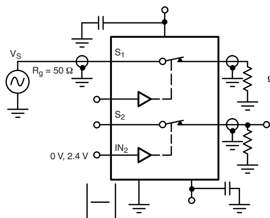
Figure 4. Channel-to-Channel Crosstalk
