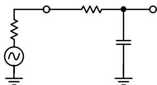
Fig. 5 - Simplified Model of One Multiplexer Channel
