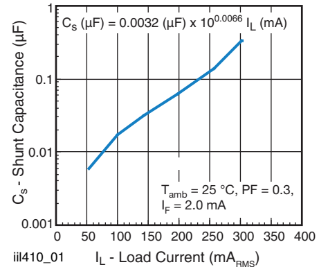
Fig. 13 - Shunt Capacitance vs. Load Current
