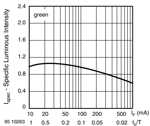
Fig. 11 - Specific Luminous Intensity vs. Forward Current
