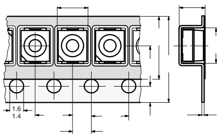
Fig. 9 - Tape Dimensions in mm for PLCC-2
