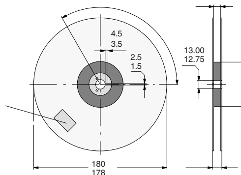
Fig. 11 - Dimensions of Reel-GS08
