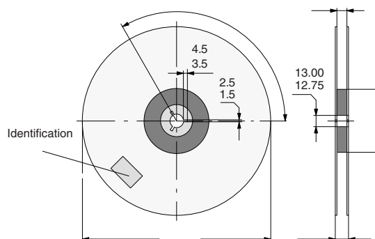
Fig. 12 - Dimensions of Reel-GS18
