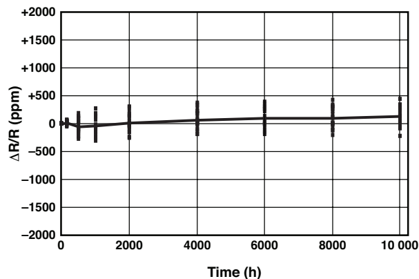
FIGURE 3 – 1240W 10 K \Omega LOAD LIFE, 20 UNITS, 10 000 h at .25 W, +85°C (Wiper at CW)
