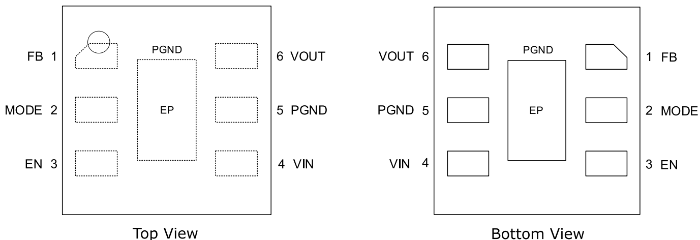
Figure 1: Pinout
