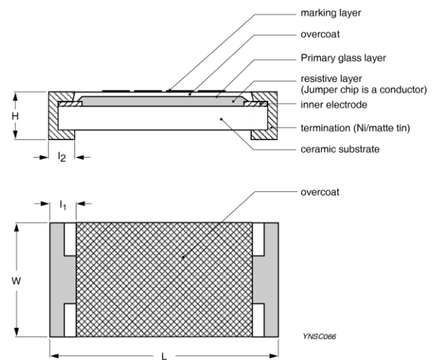
Fig. 3 Chip resistor outlines
